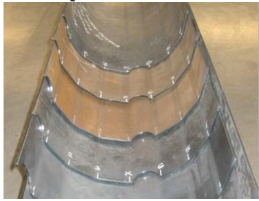
Polygonal Poles
